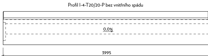
Pohled "a"
