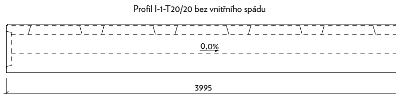
Pohled "a"
