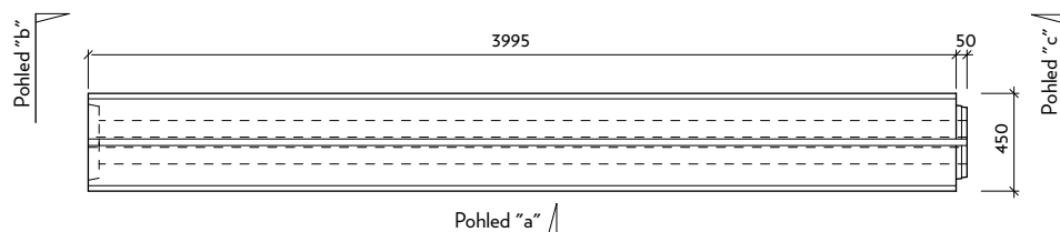
Pohled "a"
