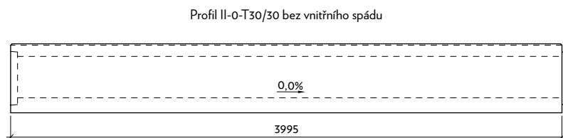
Pohled "a"
