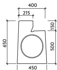
Pohled "a"
