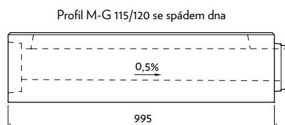
Pohled "a"
