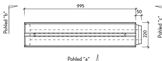
Pohled "a"
