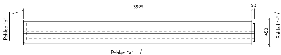
Pohled "a"
