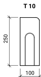
Bokorys
