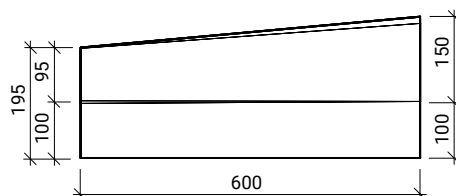
Pohled "c"
