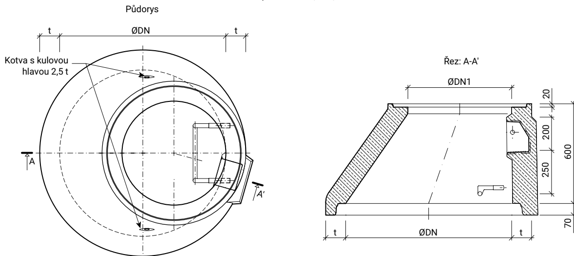
TBR-Q.1 1000x625/600/120 SPK
