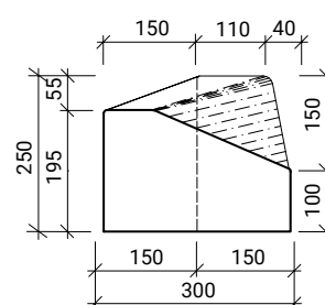
Pohled "a"
