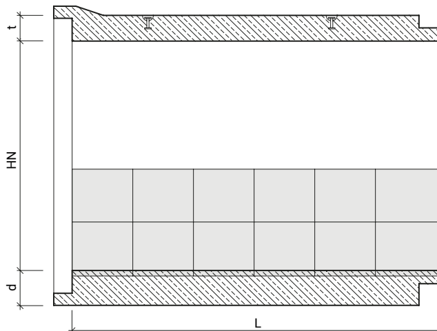
TZO-Q 700x1250/2000/140 PN II XA3 D OC DEHA
