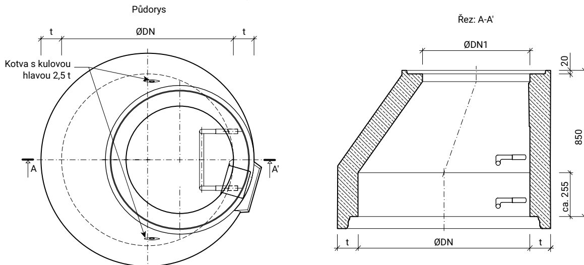
TBR - Q.1 1000x625/850/120 SPK DEHA
