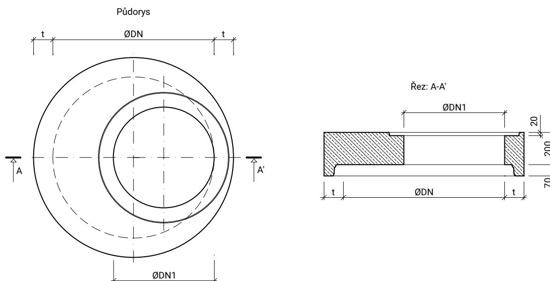
LS01 - TZK-Q.1 1000x625-200 D400(B125)
