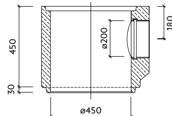
TBV-Q 450/450/3d PVC
