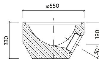
TBV-Q 450/330/1a PVC
