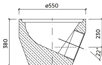
TBV-Q 450/380/1d PVC
