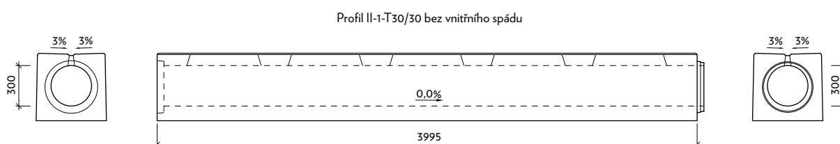
Pohled "a"
