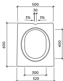
Pohled "a"="b" III-O-CS - pero/pero
